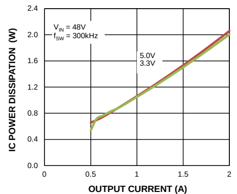
IC Power Dissipation vs. Output Current MIC28512-1
