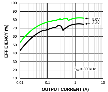
Efficiency ( V_{IN} = 48V ) vs. Output Current MIC28512-1
