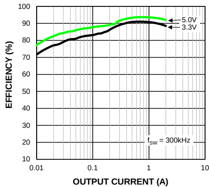
Efficiency ( V_{IN} = 12V ) vs. Output Current MIC28512-1
