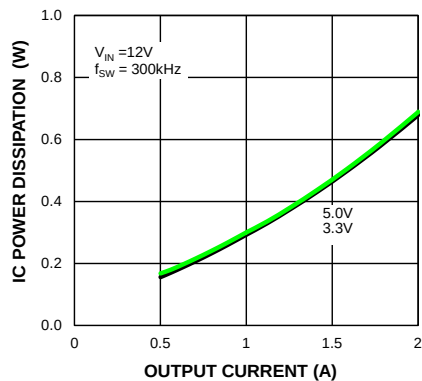
IC Power Dissipation vs. Output Current MIC28512-1
