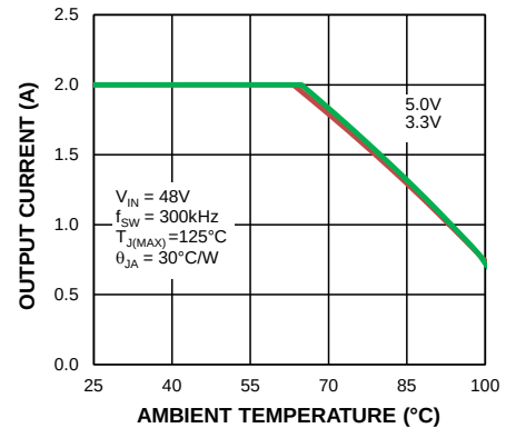
48V Input Thermal Derating MIC28512-1
