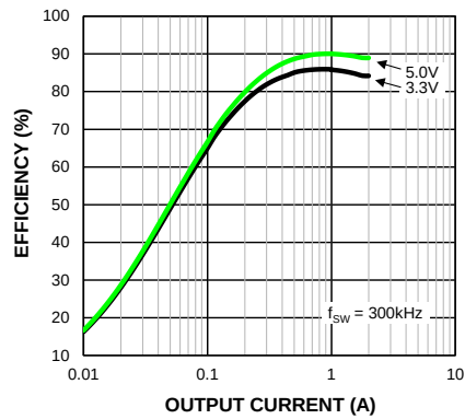
Efficiency (VIN = 24V) vs. Output Current MIC28512-2
