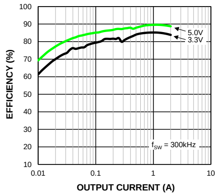
Efficiency ( V_{IN} = 24V ) vs. Output Current MIC28512-1
