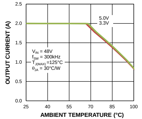
48V Input Thermal Derating MIC28512-2
