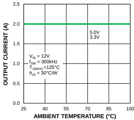
12V Input Thermal Derating MIC28512-1
