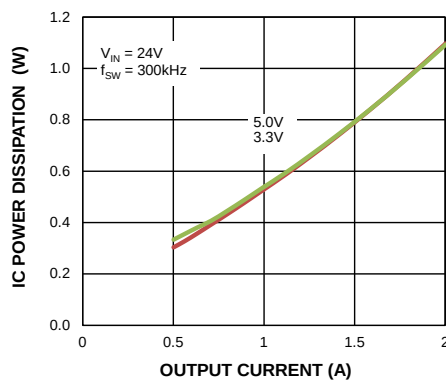
IC Power Dissipation vs. Output Current MIC28512-1
